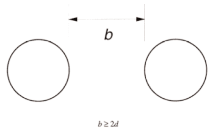
Figure 14 — Relationship between two holes
