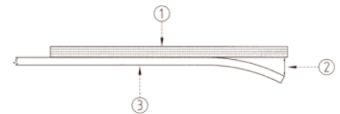
Figure 4 — Representation of roller wave distortion
