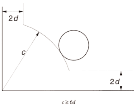
Figure 15 — Relationship between hole and corner of pane
