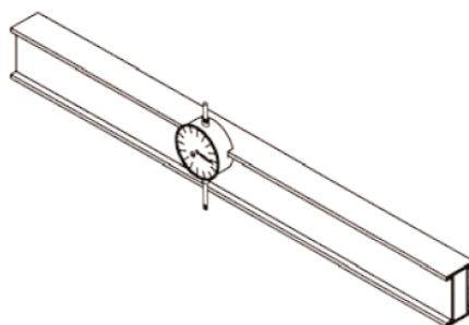
Figure B.1 — Roller wave measurement apparatus
