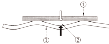
Key: 1 - straight edge 2 - roller wave distortion 2 - thermally toughened glass
