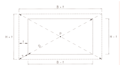
Figure 2 — Tolerance limits for dimensions of rectangular panes
