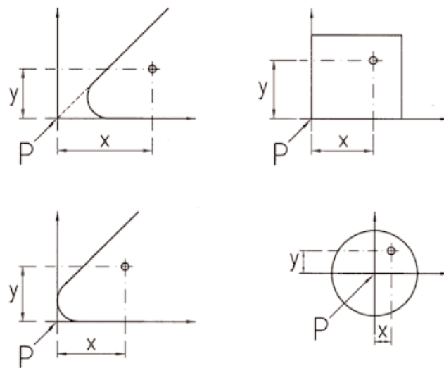
Figure 16 — Examples of the positioning of holes relative to the datum point
