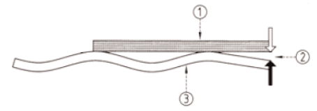
Key: 1 - straight edge 2 - edge lift 2 - thermally toughened glass
