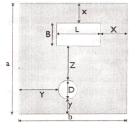
Figure 18b — Examples of cut-outs
