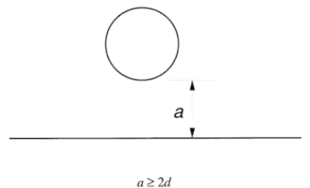
Figure 13 — Relationship between hole and edge of pane
